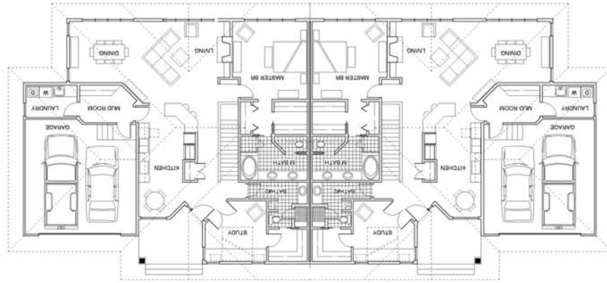
FIRST FLOOR PLAN @ 1/32=1'-0"
